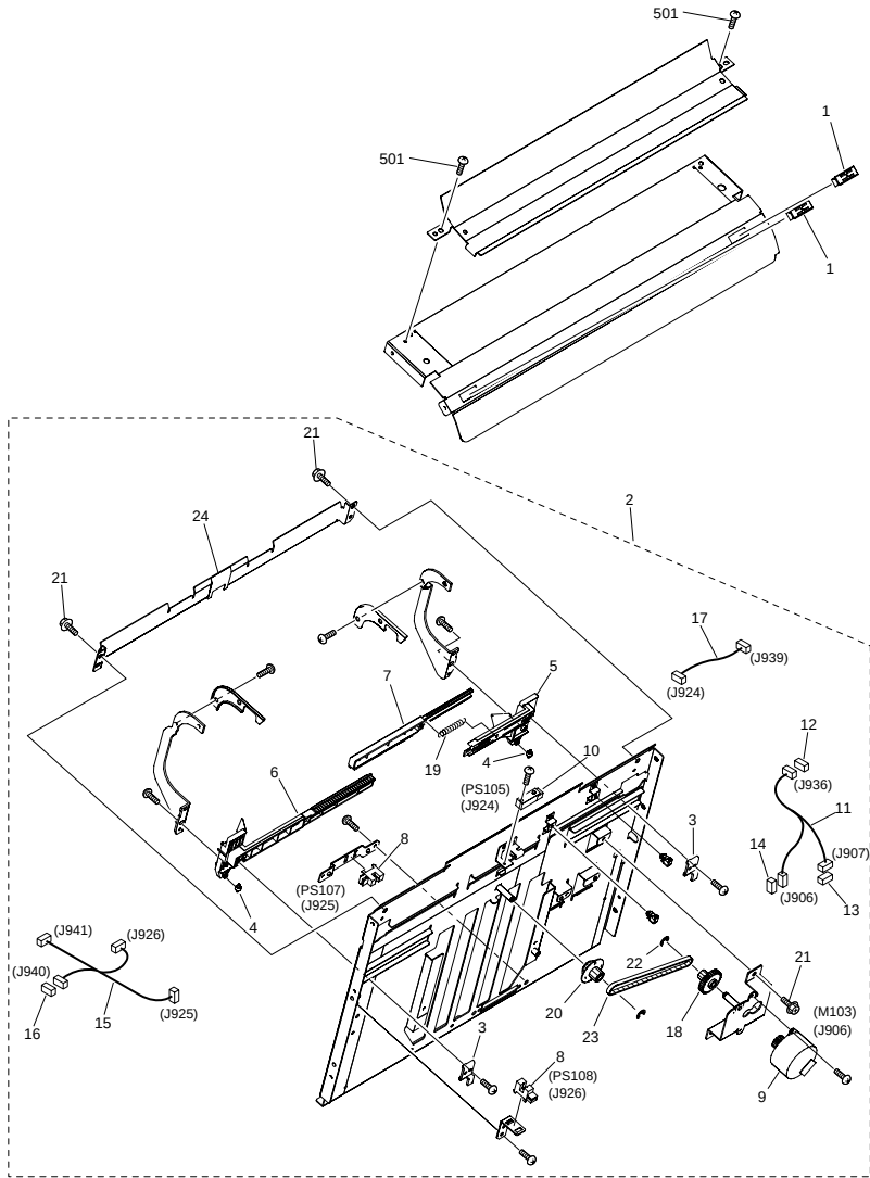
FIGURE Q56 SADDLE PATH GUIDE ASSEMBLY
