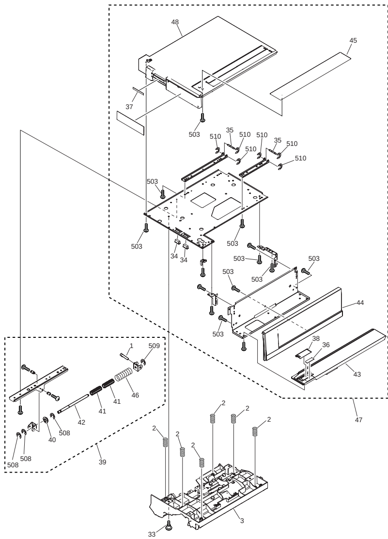
FIGURE Q37 UPPER FEEDER ASSEMBLY
