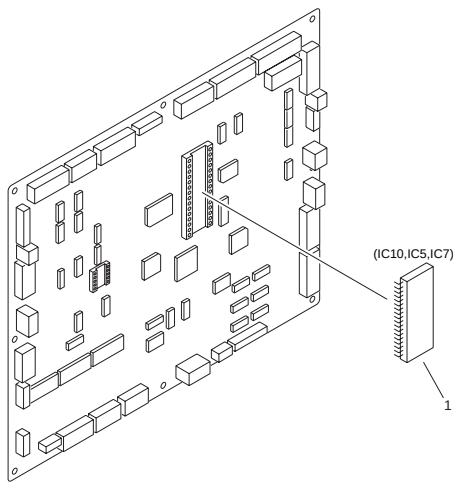
FIGURE Q90 FINISHER CONTROLLER PCB ASS'Y
