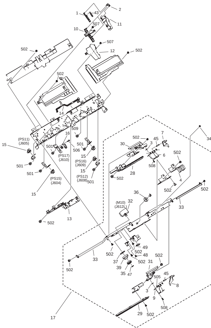
FIGURE Q21 OPERATION TRAY ASSEMBLY
