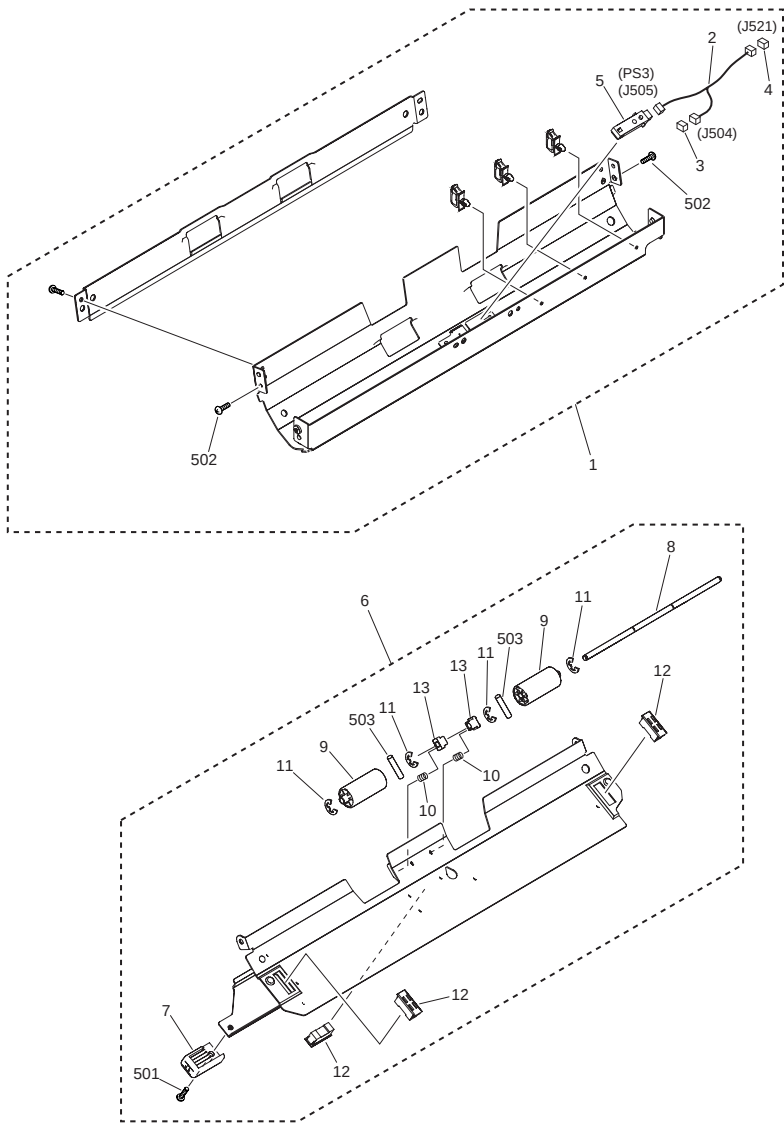
FIGURE Q32 ENTRANCE GUIDE ASSEMBLY
