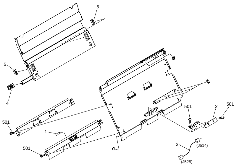
FIGURE Q31 CABLE FEEDER GUIDE ASS'Y
