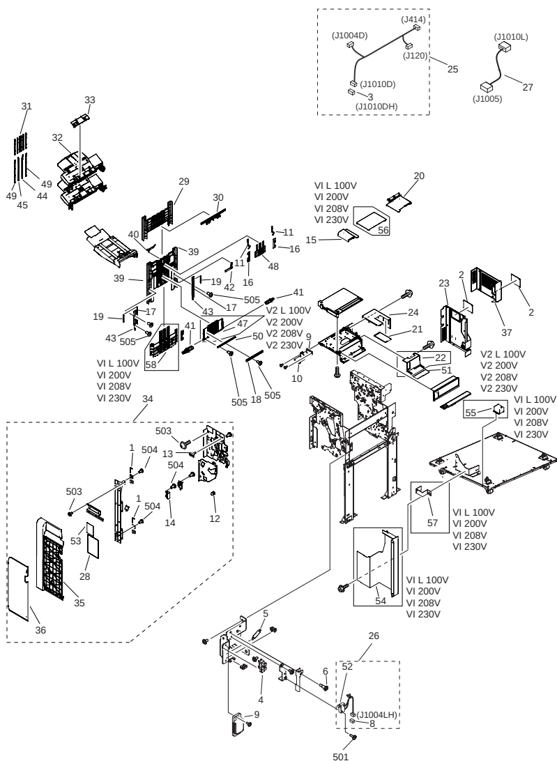
FIGURE Q10 EXTERNAL COVERS, PANELS, ETC.
