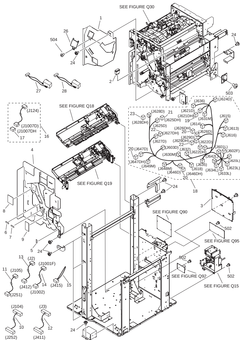
FIGURE Q11 INTERNAL COMPONENTS 1
