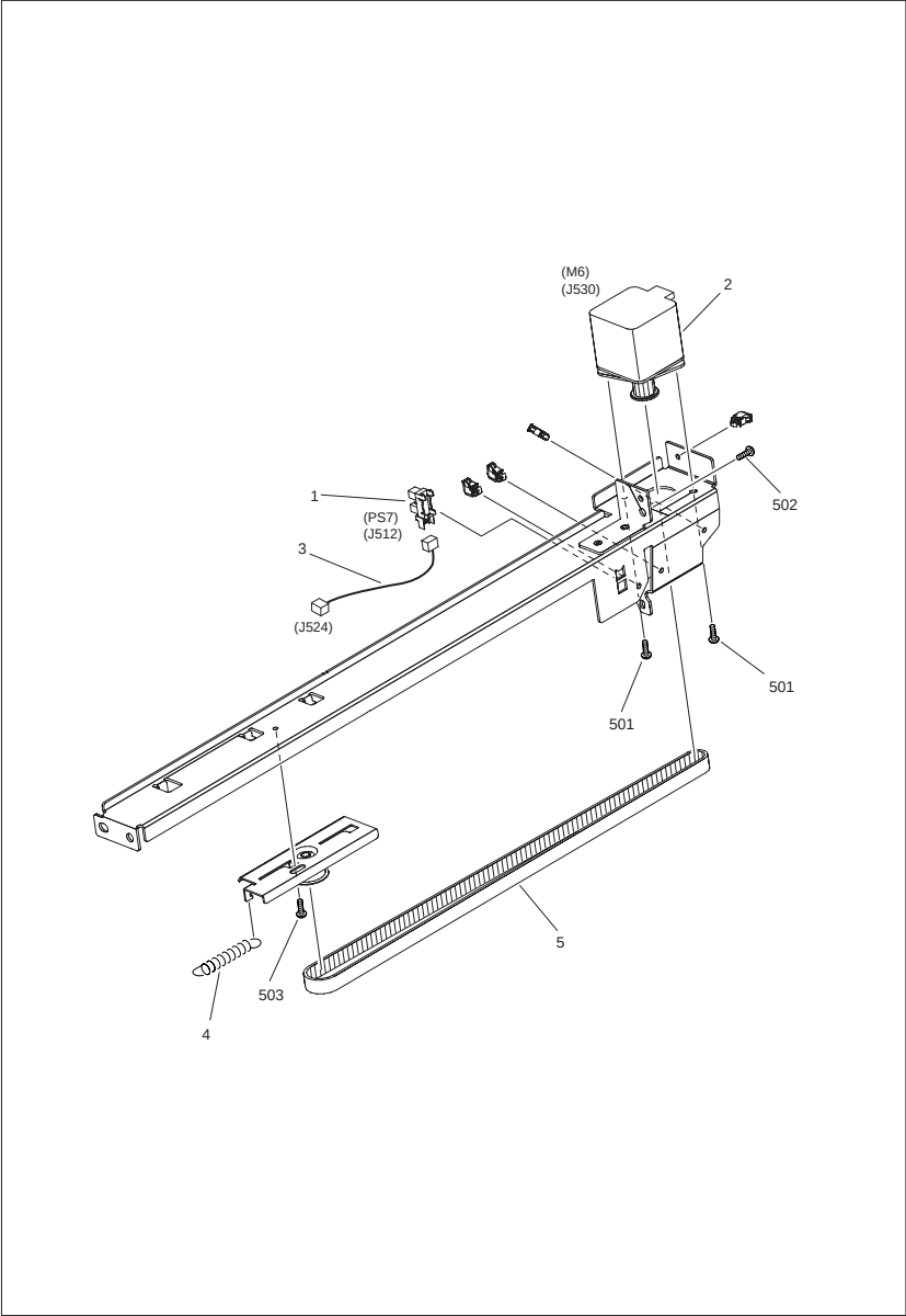
FIGURE Q38 DETECT DRIVE ASSEMBLY
