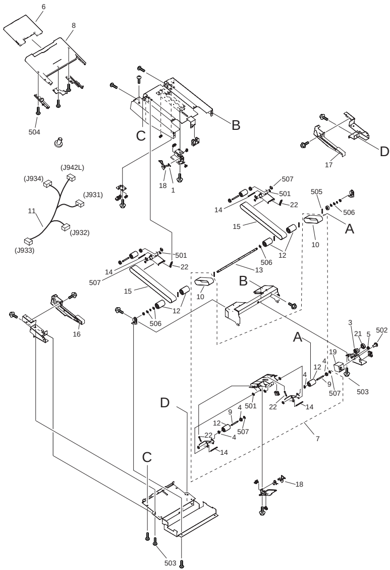
FIGURE Q14 SADDLE DELIVERY TRAY ASSEMBLY
