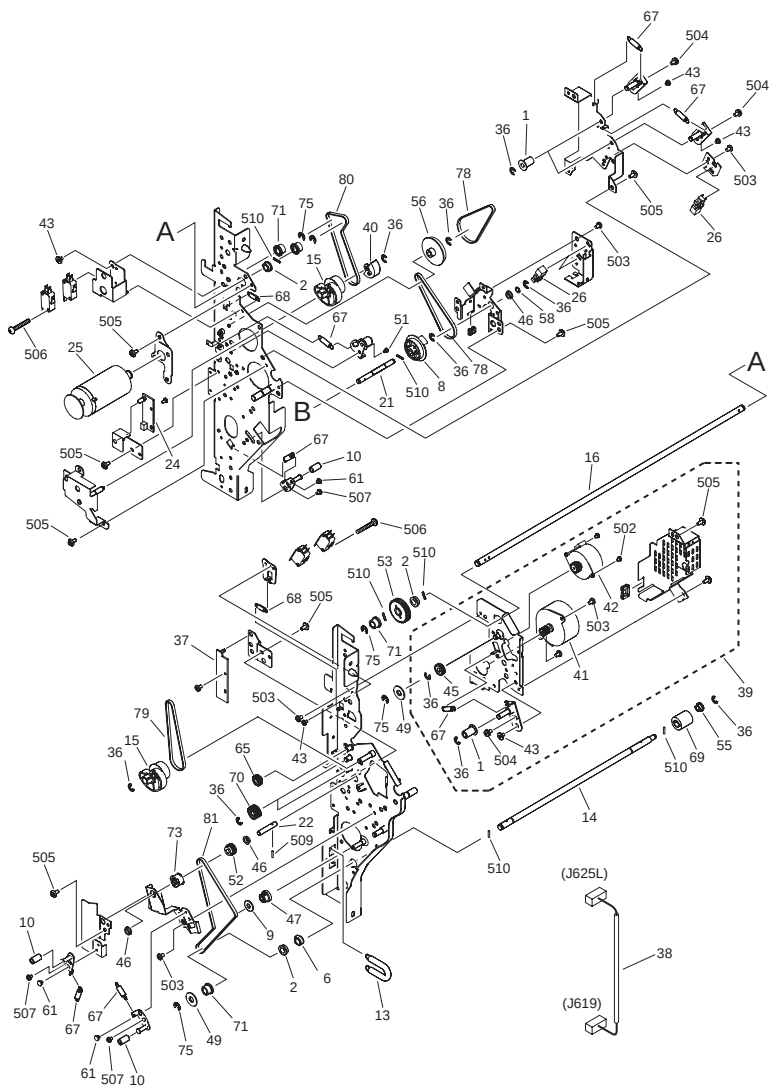
FIGURE Q20 OPERTTION ASSEMBLY
